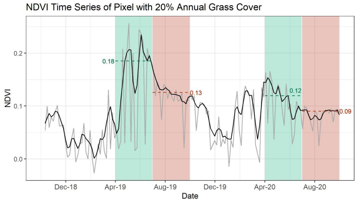
Figure 2. Two years of NDVI values at a location with 20% median annual grass cover. The raw NDVI data are shown in light grey. A smoothed time series is shown in black using the Savitzky-Golay smoothing, which performs a local polynomial regression on a series of values which are treated as being equally spaced to determine the smoothed value for each point. The shaded areas illustrate the difference between spring growth (green) and summer senescence (red) represented by NDVI to identify annual species in high-desert regions. Located in Central Nevada, from the Cortez project area, median spring NDVI at this location is greater than median summer NDVI in both 2019 and 2020 as indicated by the dashed lines.
